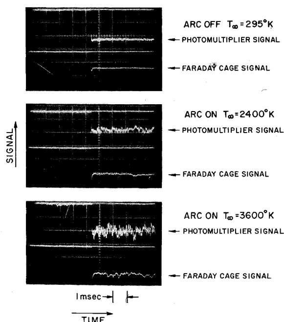
Fig. 2 Electron beam current and photomultiplier response to the N_2(2+) emission at the jet centerline. The electron beam was chopped at 100 Hz with a 50% duty cycle.
