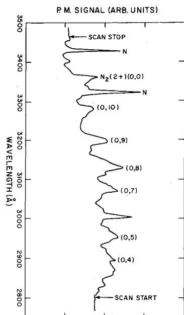
Fig. 5 Composite spectral scan of the thermal emission in the N_2 -Teflon boundary layer for the same ablation rate as in Fig. 4.
