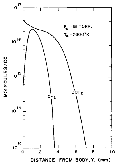
Fig. 7 Theoretical CF_2 and COF_2 concentration profiles.
