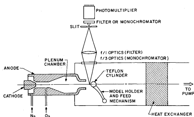
Fig. 1 Schematic of low-density arcjet and associated optical system.
