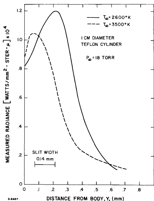
Fig. 6 CF_2 concentration profile measurements.
