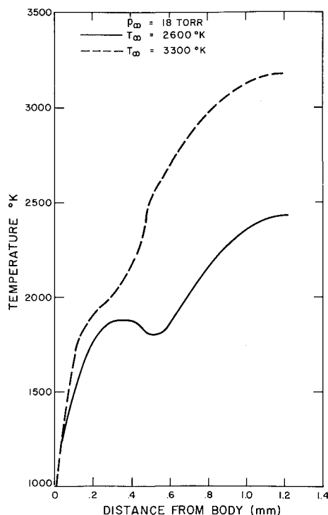
Fig. 8 Theoretical temperature profiles in the air-Teflon stagnation point boundary layer.
